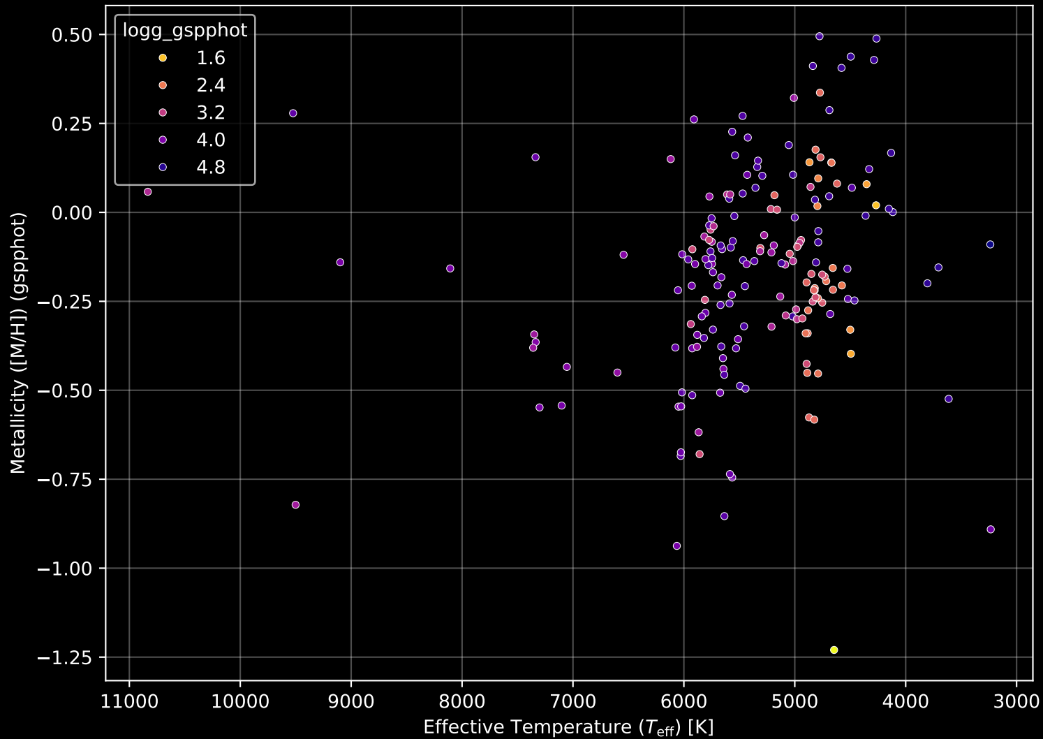
APOGEE DR17 Field: [195+28_MGA] Stellar Population Parameters (n= 187)
