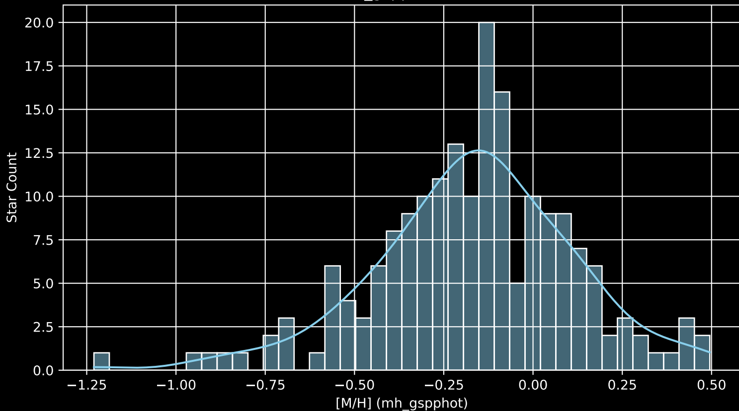
APOGEE DR17 Field: [195+28_MGA [M/H] (mh_gspphot) (n= 187)
