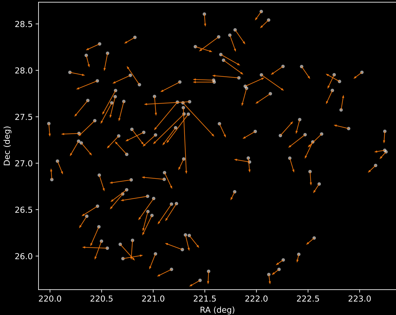
APOGEE DR17 Cluster 2 Proper Motion Vectors (n=108)
