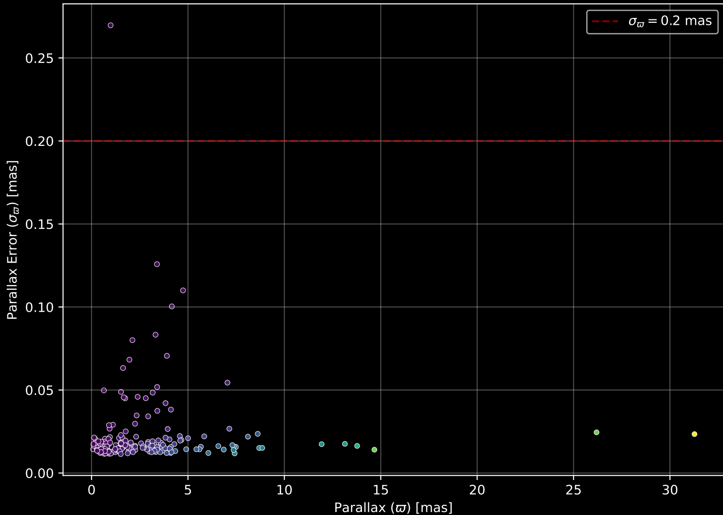
APOGEE DR17 Field: [195+28_MGA] Parallax Quality (n= 187)
