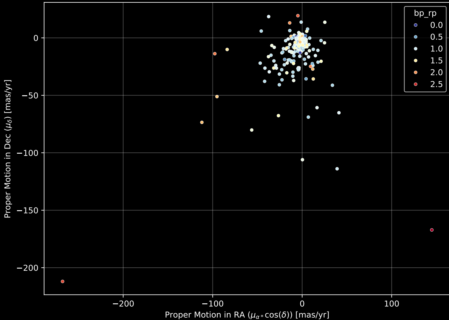
APOGEE DR17 Field: [195+28_MGA] Proper Motion Diagram (n= 187)
