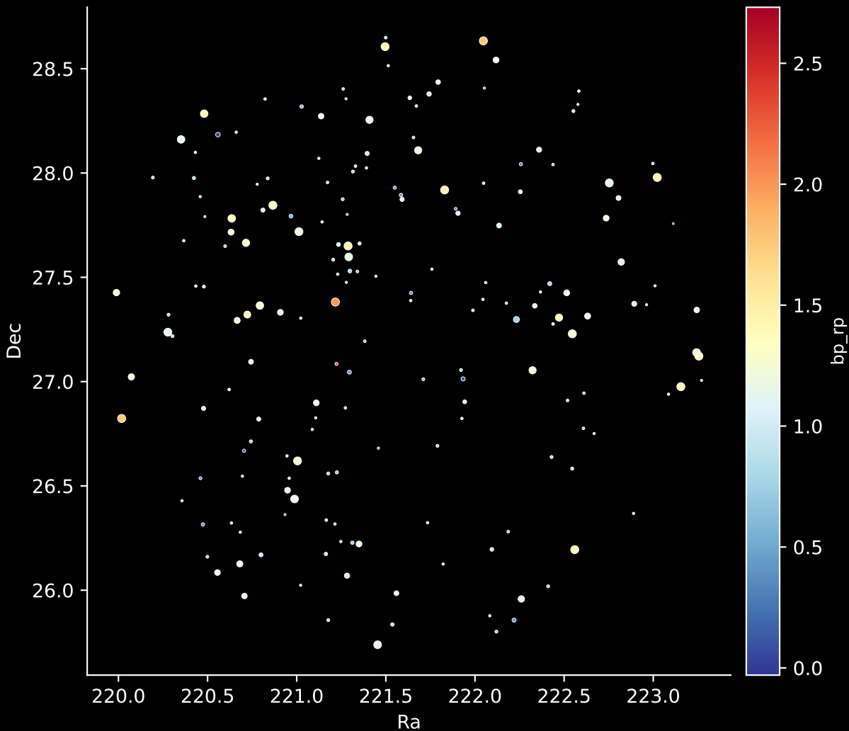
APOGEE DR17 Field: [195+28_MGA] Stars: 187
