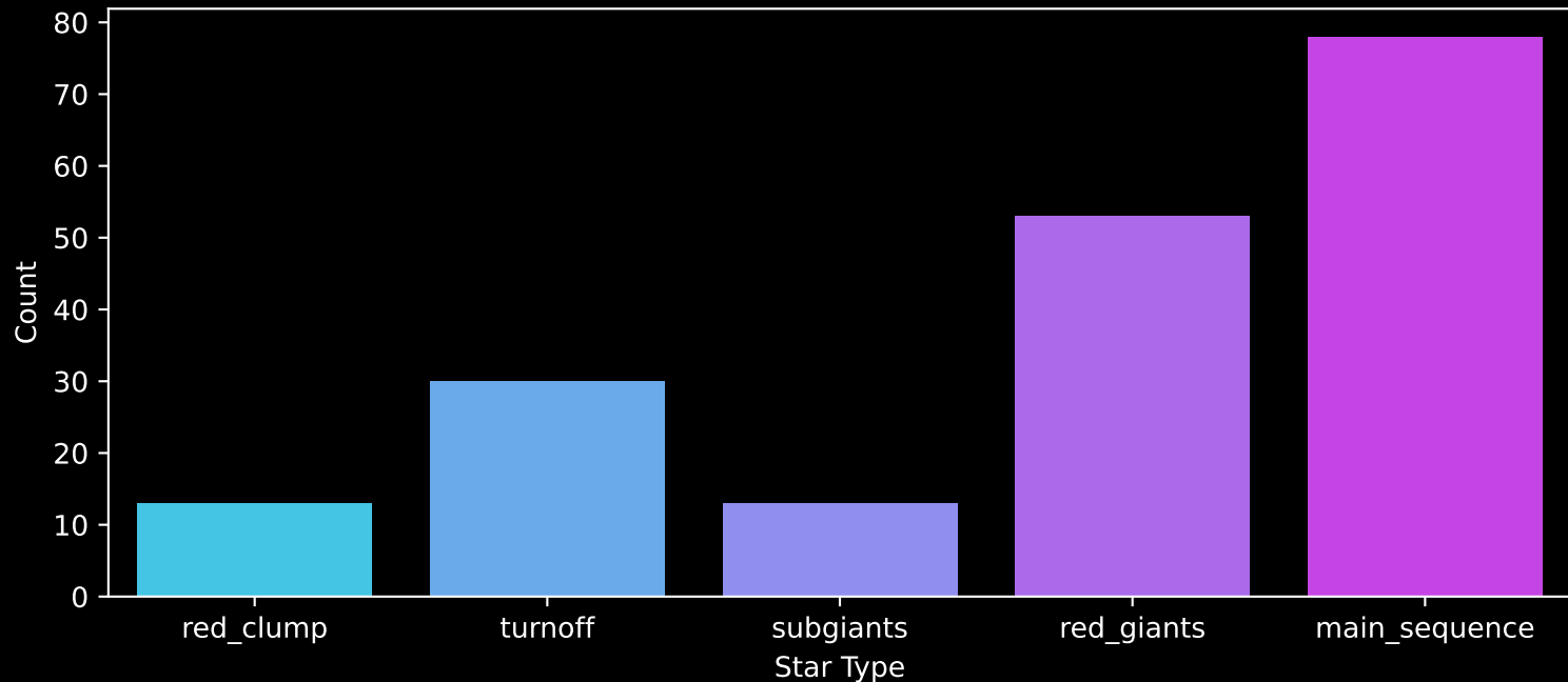
APOGEE DR17 Field: [195+28_MGA] Count plot of Star Type
