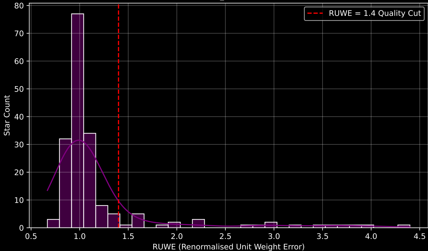
GAPOGEE DR17 Field [195+28_MGA] RUWE Distribution (n= 182)
